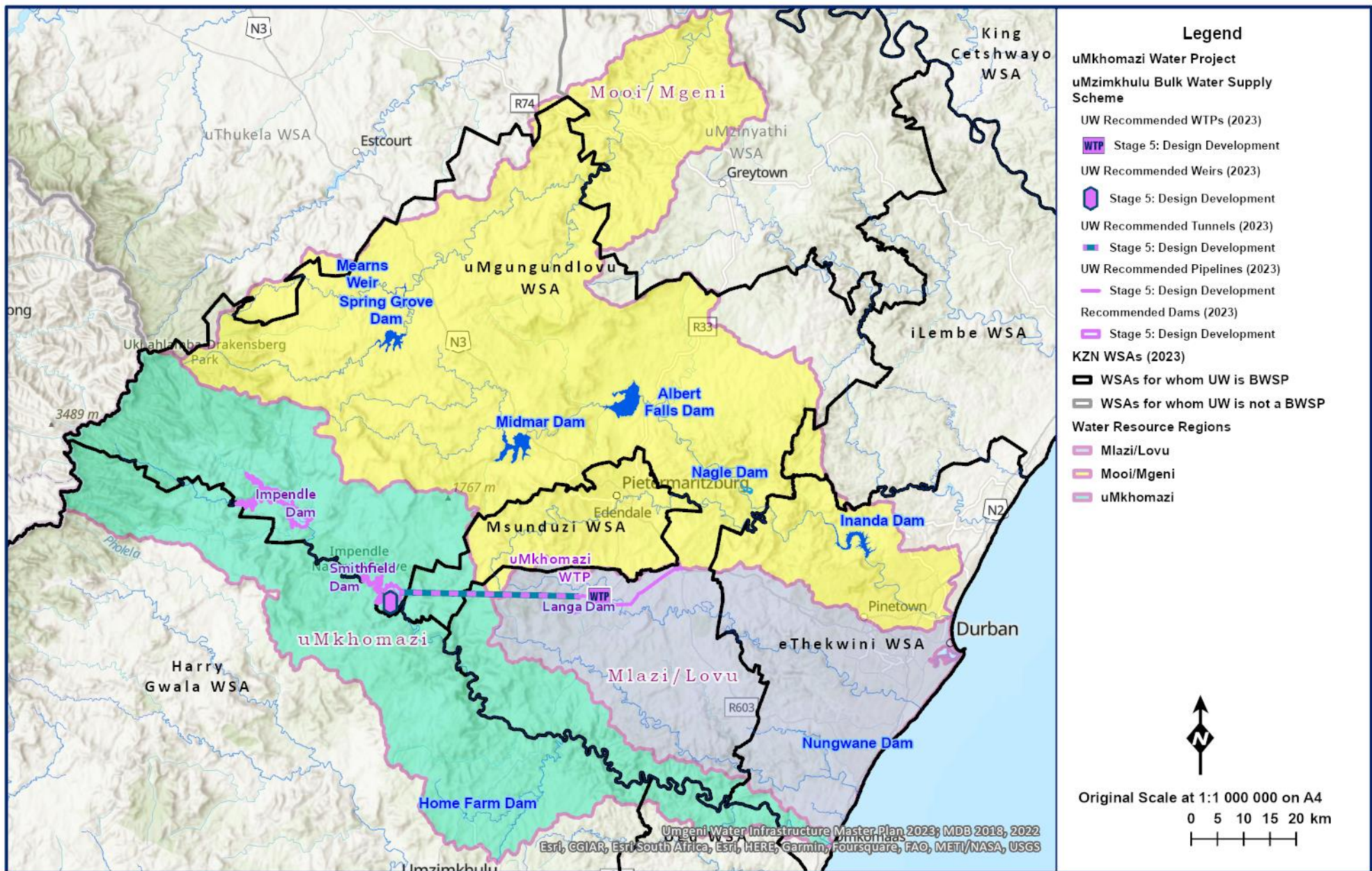
Figure 7.17 Locality map of the uMkhomazi, uMlazi and uMgeni river catchments.
