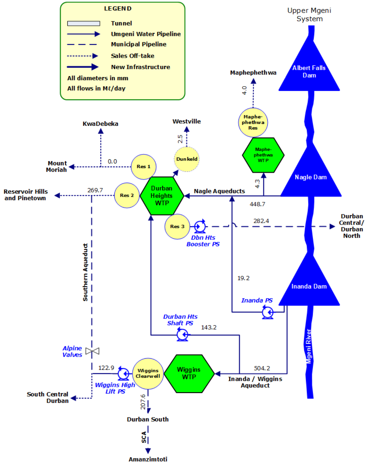
Figure 7.63 Schematic of the Lower uMgeni System.
