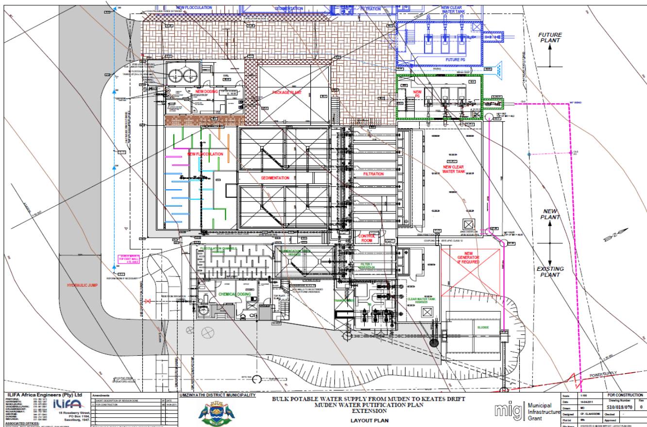
Figure 7.88 General layout of the Mudén WTP upgrade.
