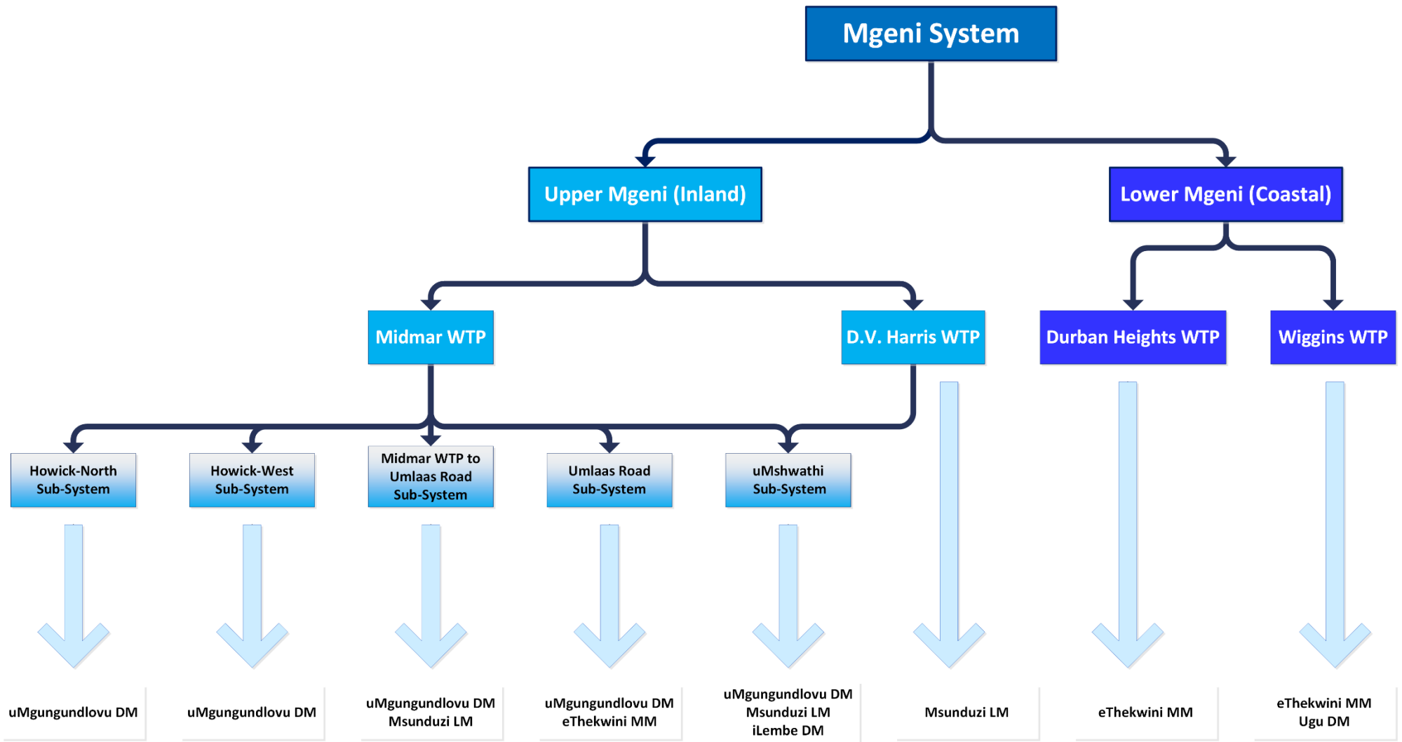
Figure 7.2 Network chart of the uMngeni System.
