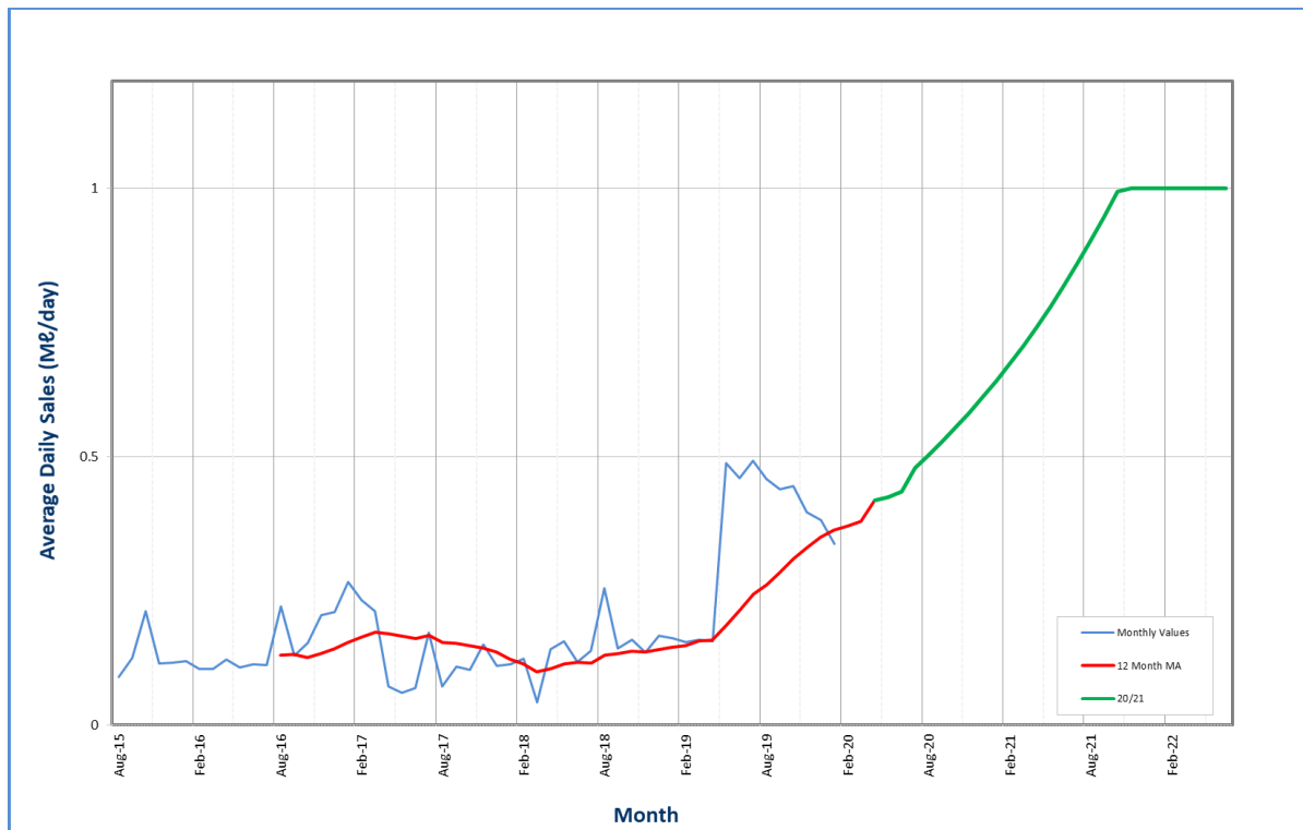
Figure 7.75 Water demand from Lidgetton WTP.
