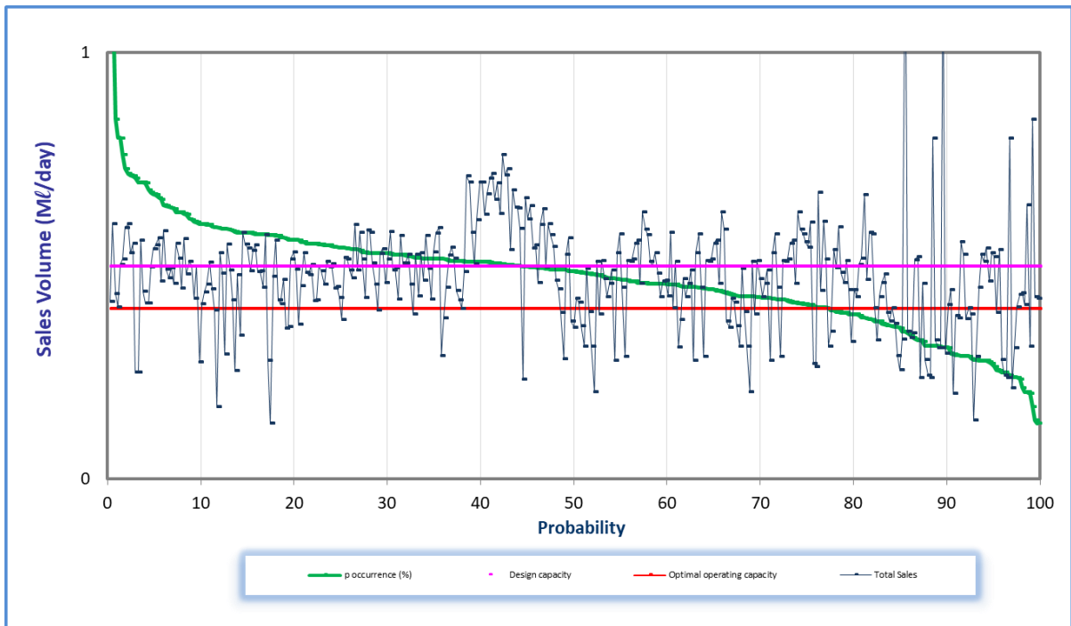
Figure 7.83 Analysis of historical production at Spring Grove WTP (November 2022 to October 2023).
