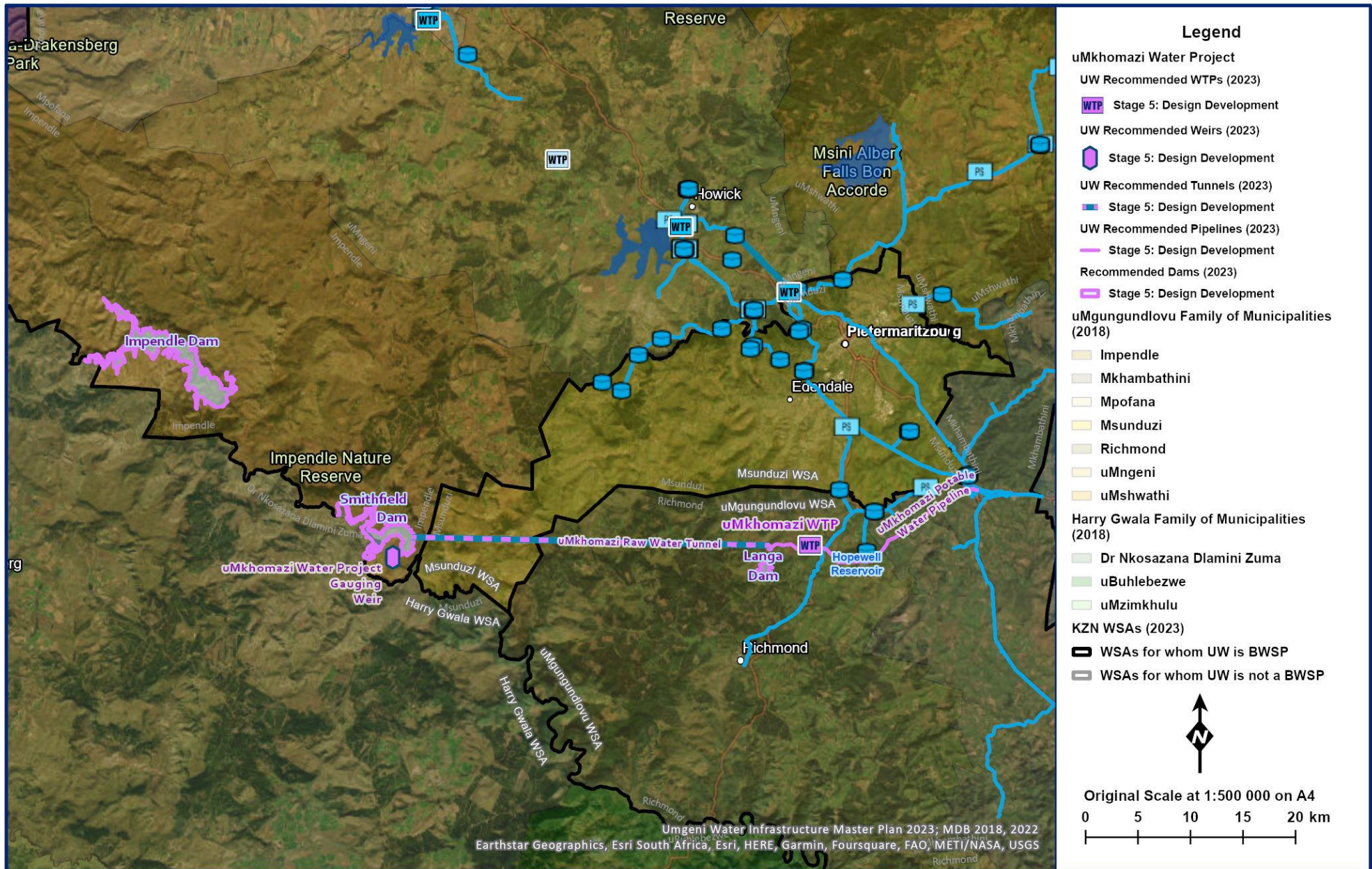
Figure 7.58 uMkhomazi Water Project.
