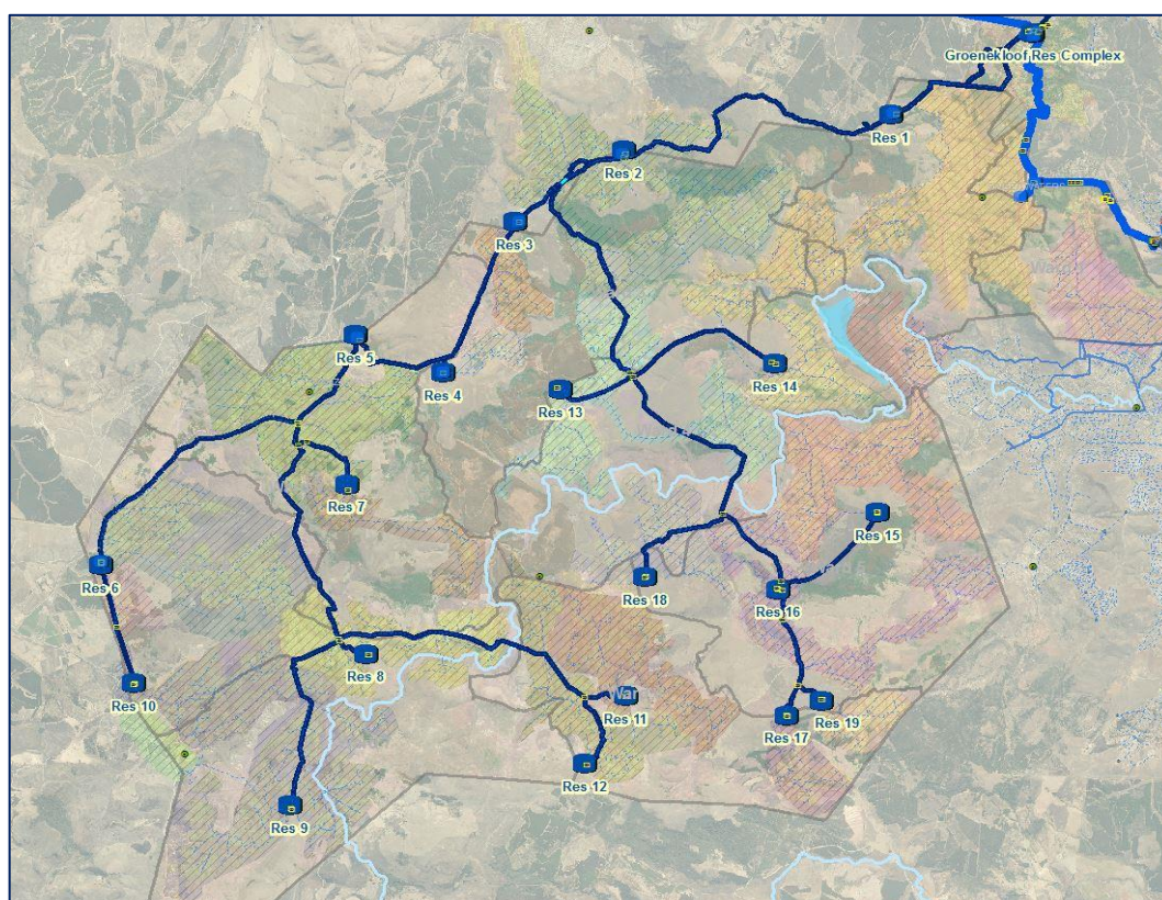
Figure 7.66 General layout of the Vulindlela System.
