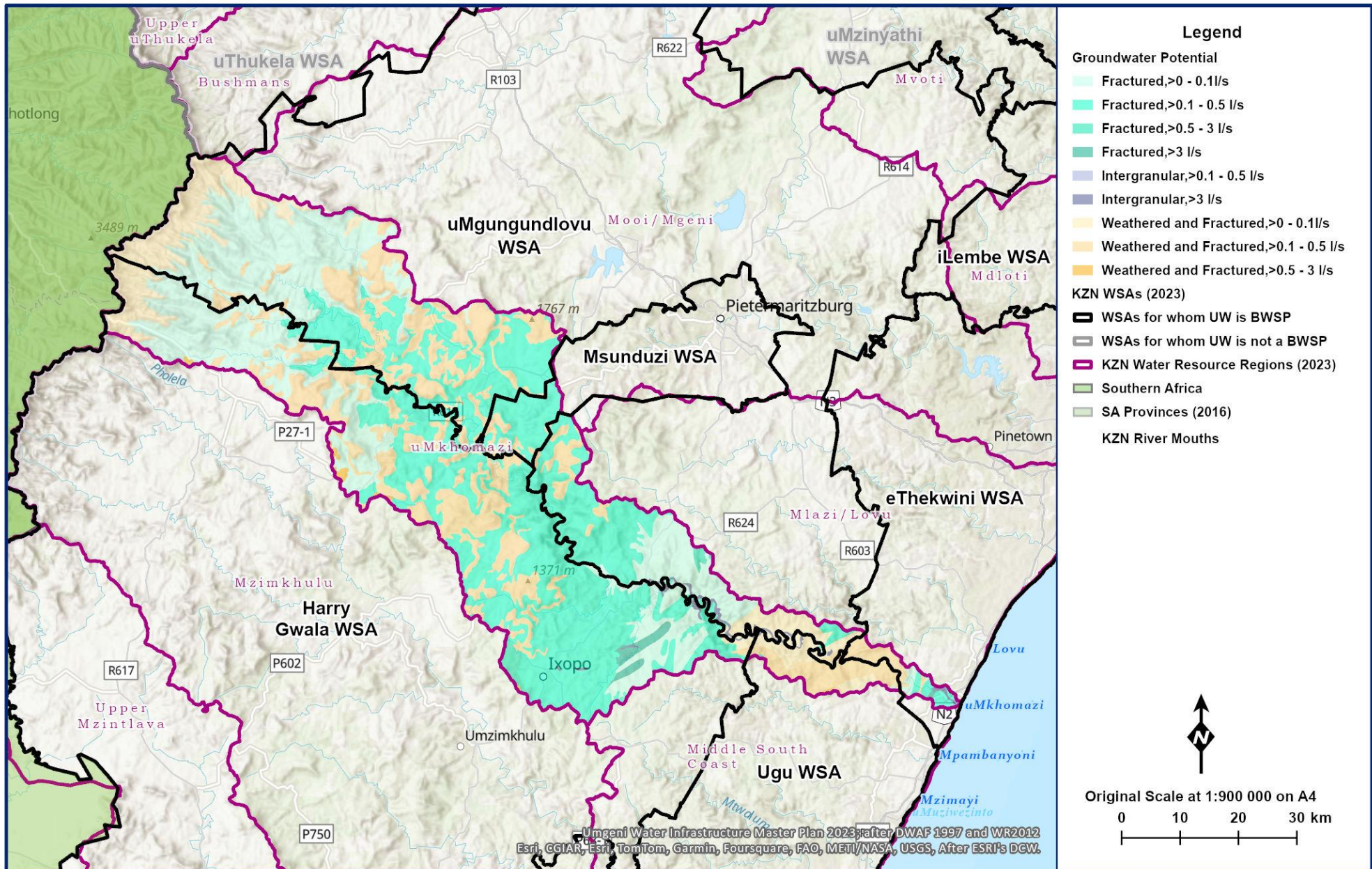
Figure 7.19 Groundwater potential in the Mkhomazi Region (after DWA 1997 and WR2012, MDB 2020, Umgeni-uThukela Water 2022).
