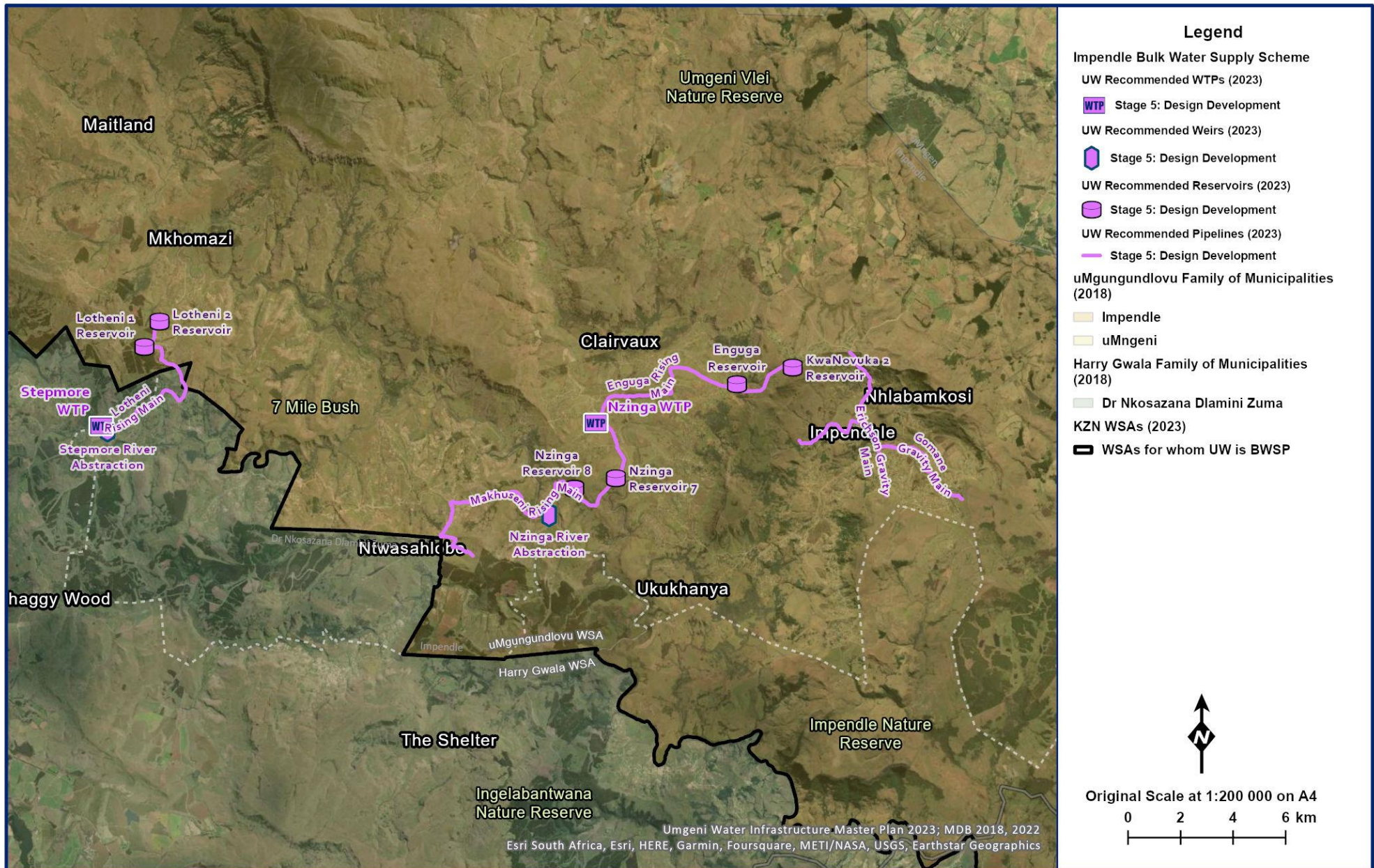
Figure 7.61 General layout of the Impendle Project Areas.
