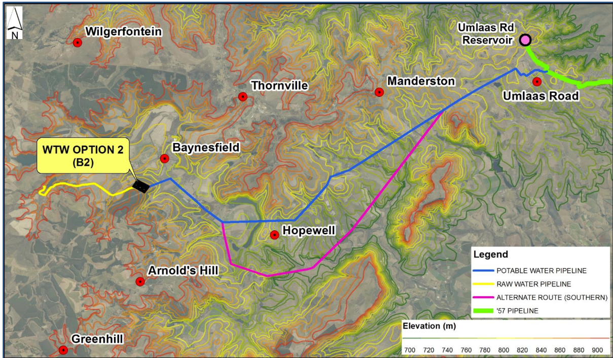
Figure 7.60 Layout of pipeline.
