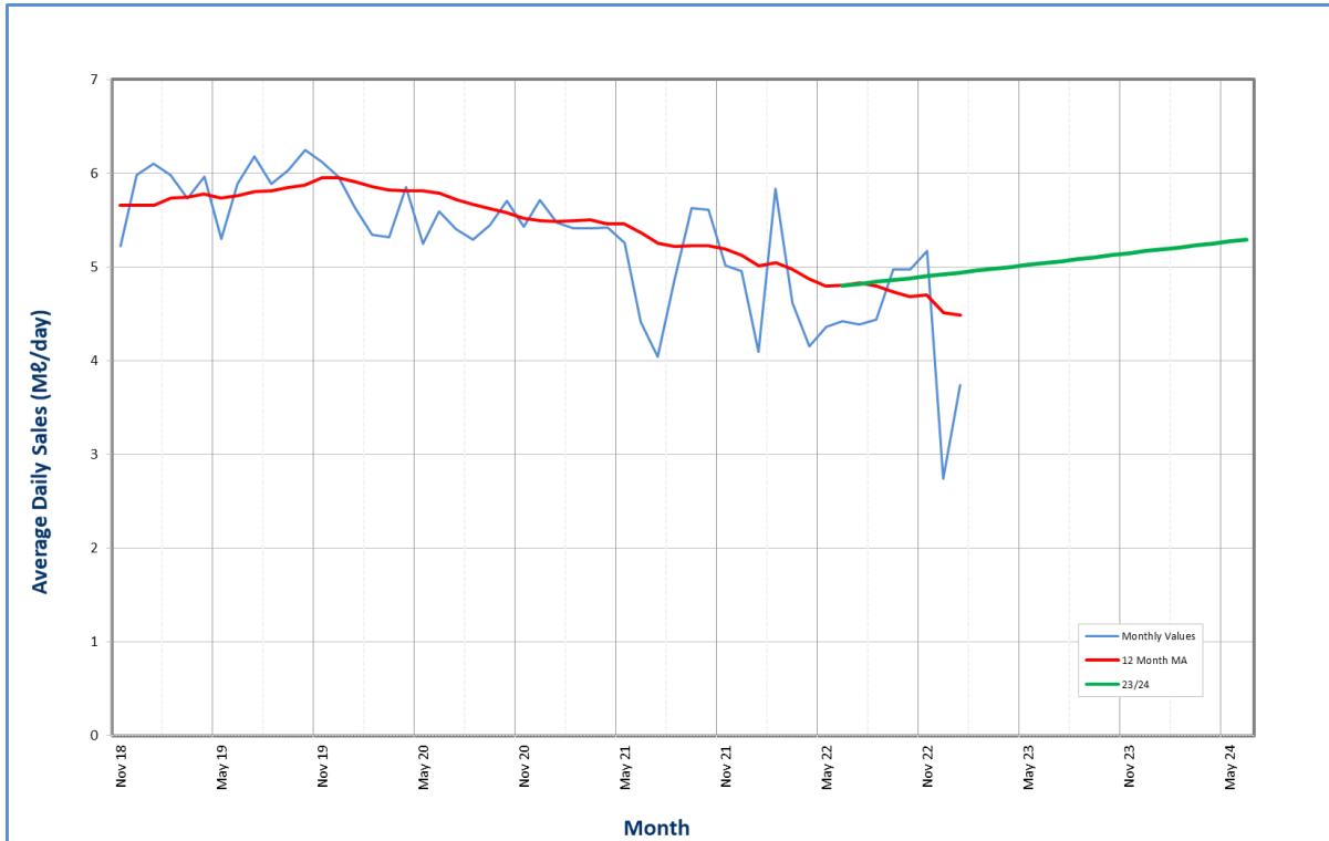
Figure 7.79 Water demand from Mpofana WTP.
