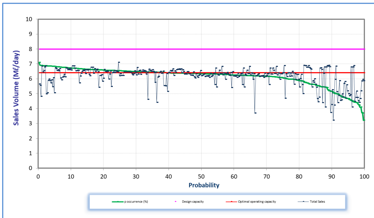
Figure 7.78 Analysis of historical production at Mpofana WTP (November 2022 to October 2023).
