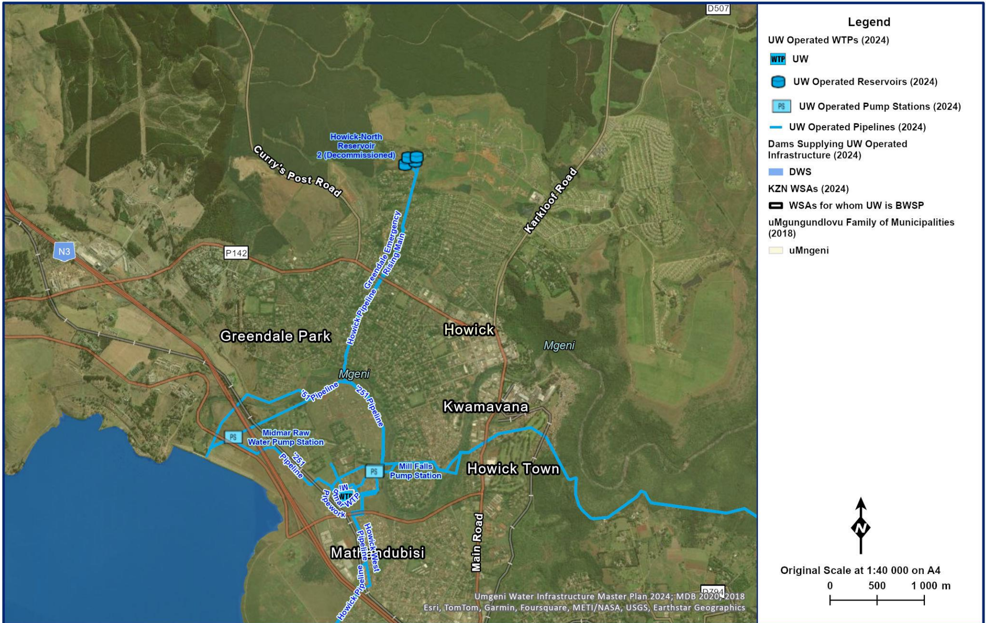
Figure 7.30 General Layout of the Howick-North Sub-System.
