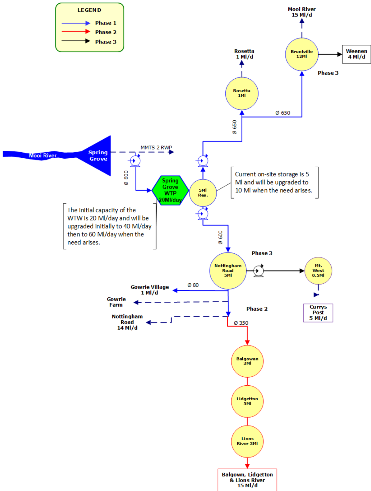
Figure 7.63 Schematic of Greater Mpofana BWSS.
