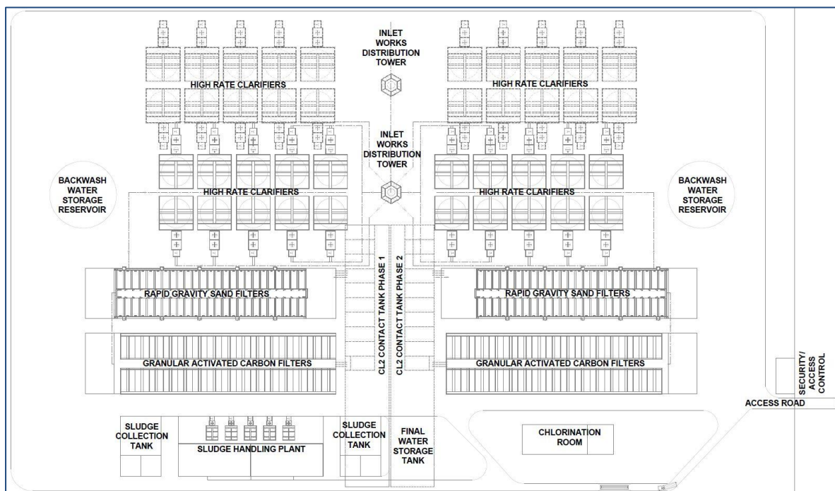
Figure 7.59 Layout of Water Treatment Plant.
