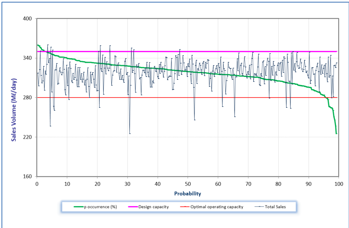
Figure 7.46 Analysis of historical production at Wiggins WTP from November 2022 to October 2023.
