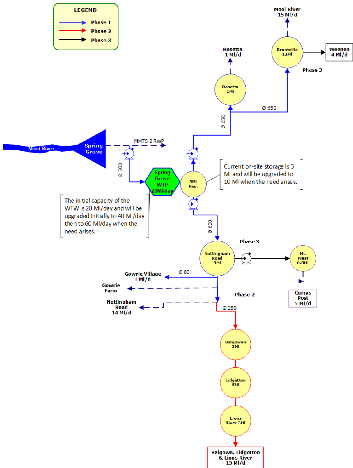
Figure 7.82 Schematic of the Spring Grove WTP System (subject to verification).
