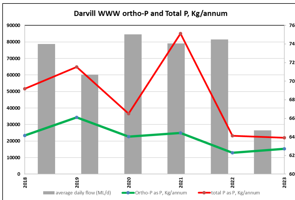
Figure 7.16 Phosphorus loads - Darvill WWW effluent.
