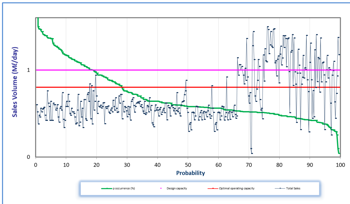
Figure 7.74 Analysis of historical production at Lidgetton WTP (November 2022 to October 2023).
