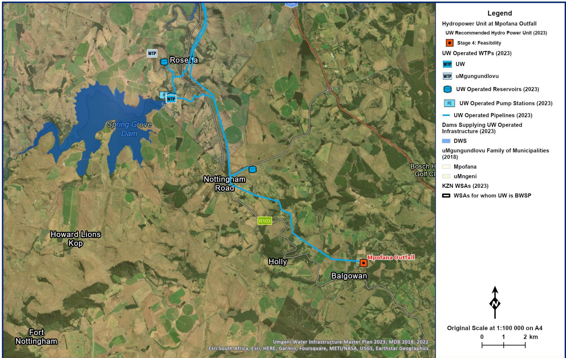
Figure 7.69 Layout of the proposed hydropower unit at the Mpofana Outfall.
