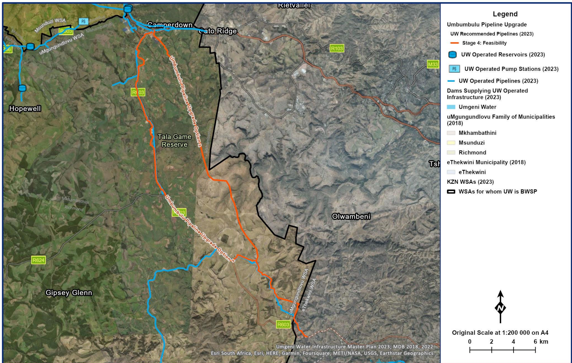
Figure 7.65 General layout of the Umbumbulu Pipeline Upgrade.
