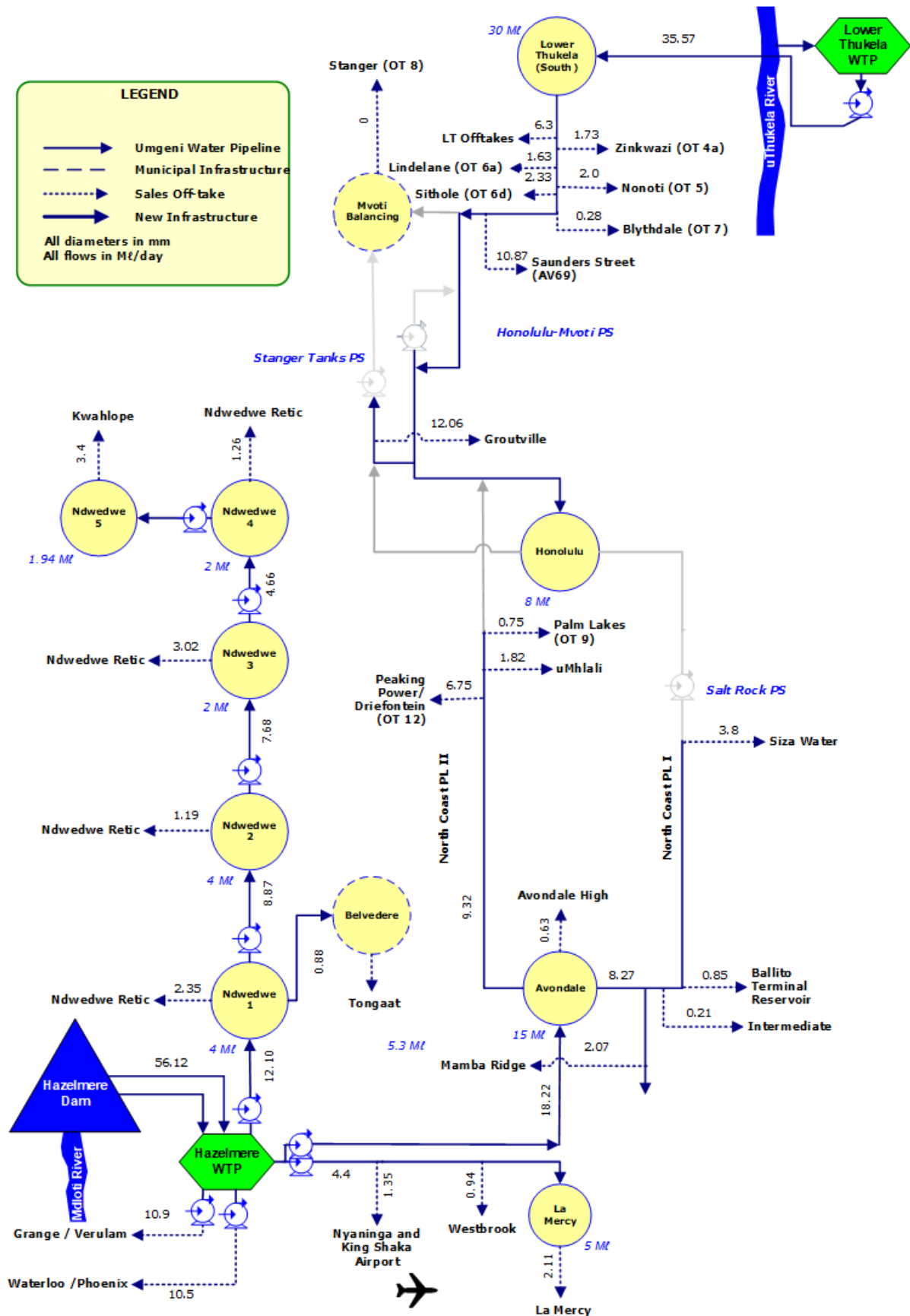
Figure 12.33 Demand on the North Coast Supply System as at October 2021.
