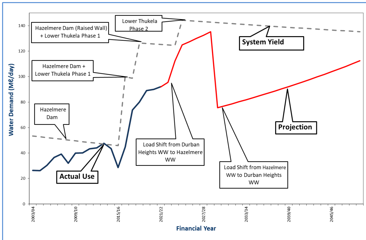
Figure 12.38 Hazelmere System Balance
