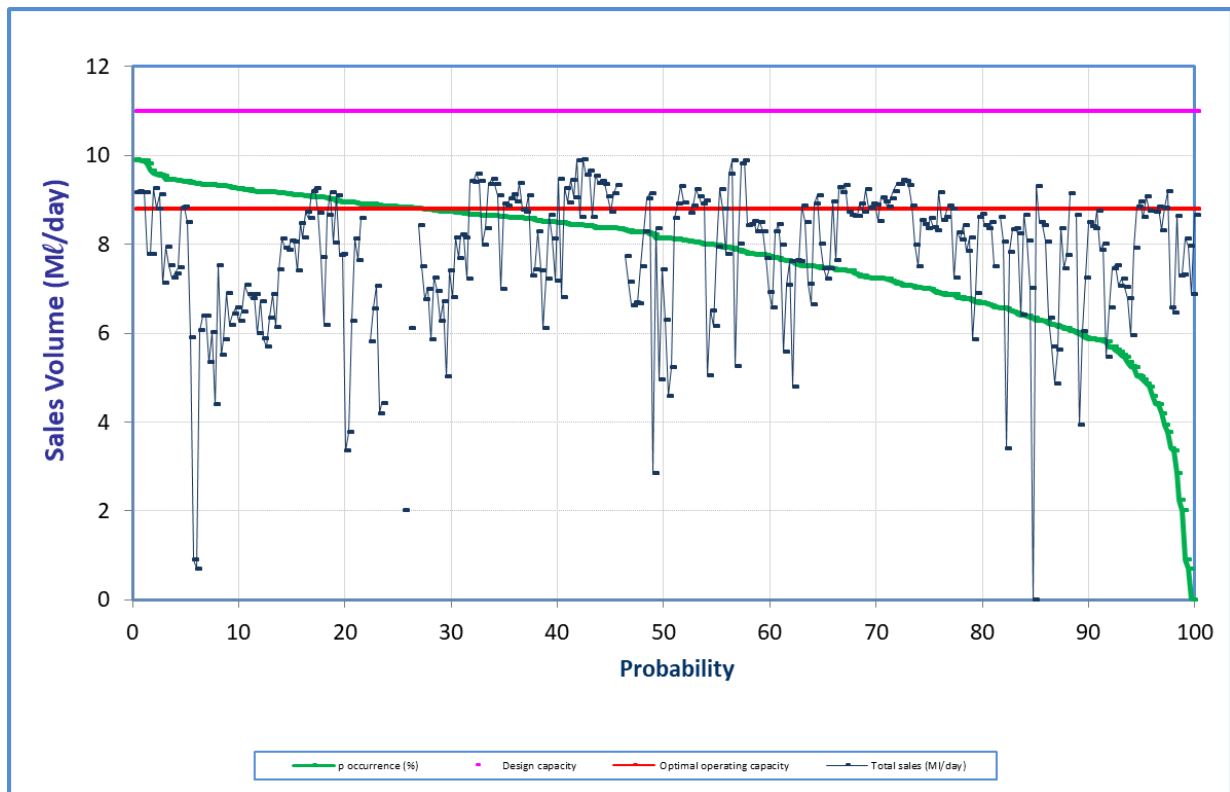
Figure 12.32 Analysis of historical production at Maphumulo WTP (November 2020 to October 2021).
