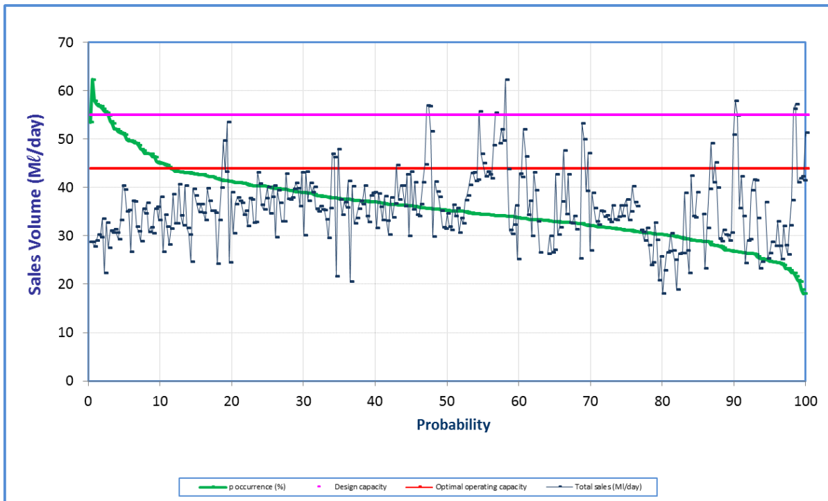
Figure 12.30 Analysis of historical production at Lower Thukela WTP (November 2020 to October 2021).
