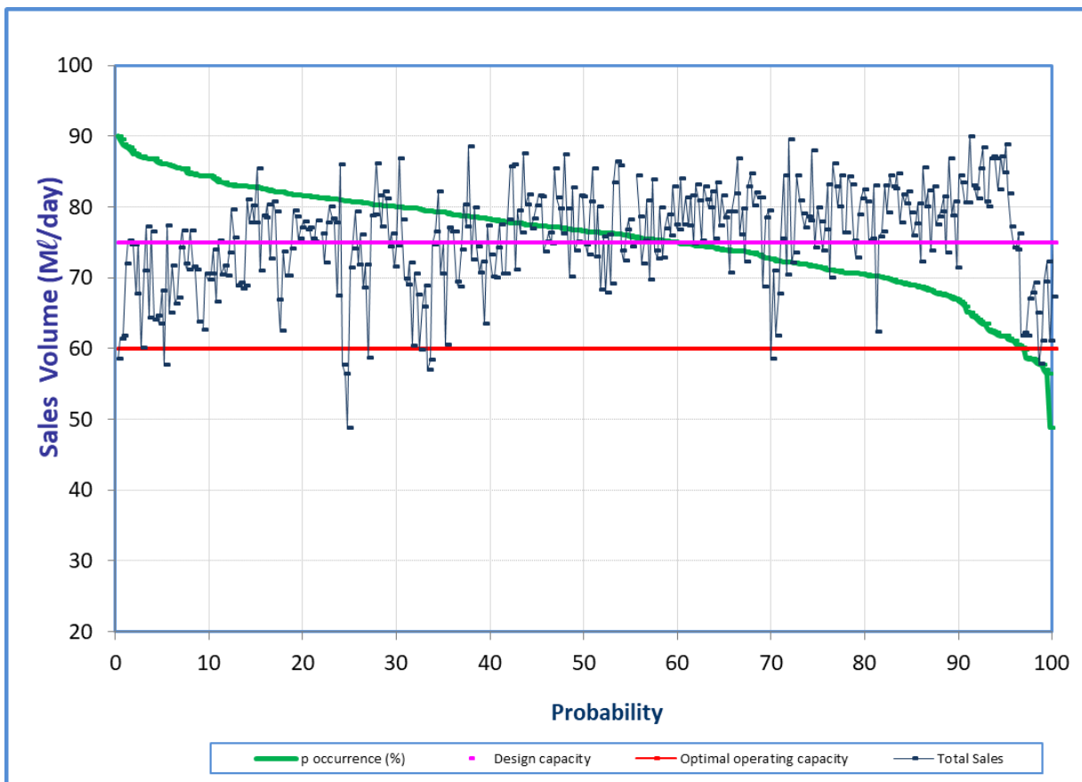
Figure 12.28 Analysis of historical production at Hazelmere WTP (November 2020 to October 2021).
