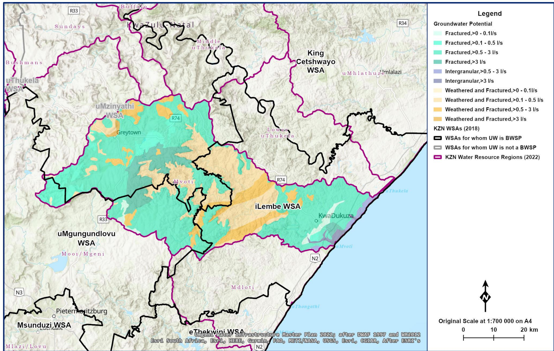
Figure 12.6 Groundwater potential in the Mvoti region (MDB 2020; Umgeni Water 2022; after DWA 1997 and WR2012).
