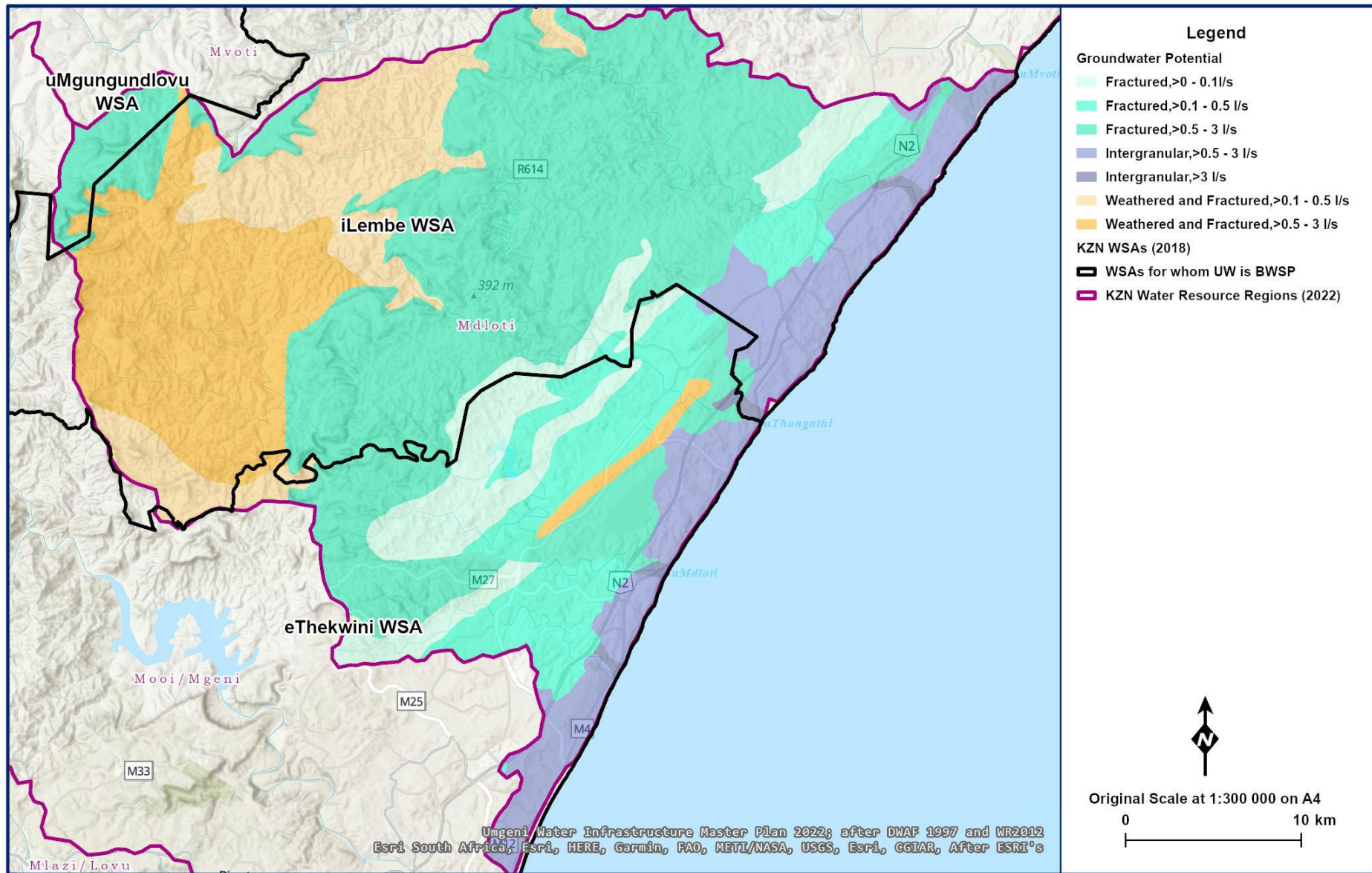
Figure 12.9 Groundwater potential in the Mdloti Region (MDB 2020; Umgeni Water 2022; after DWA 1997 and WR2012).
