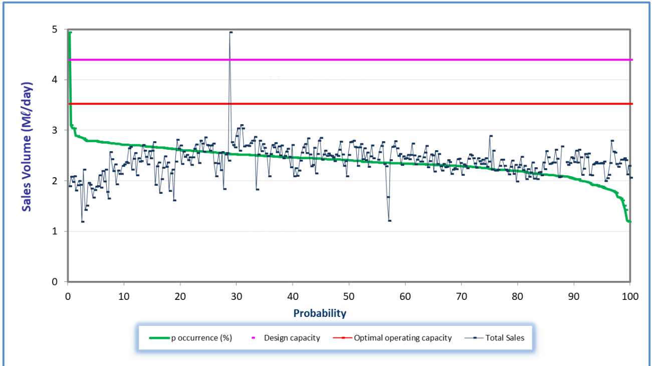
Figure 8.7 Analysis of historical production at Ixopo WTP (November 2020 to October 2021).
