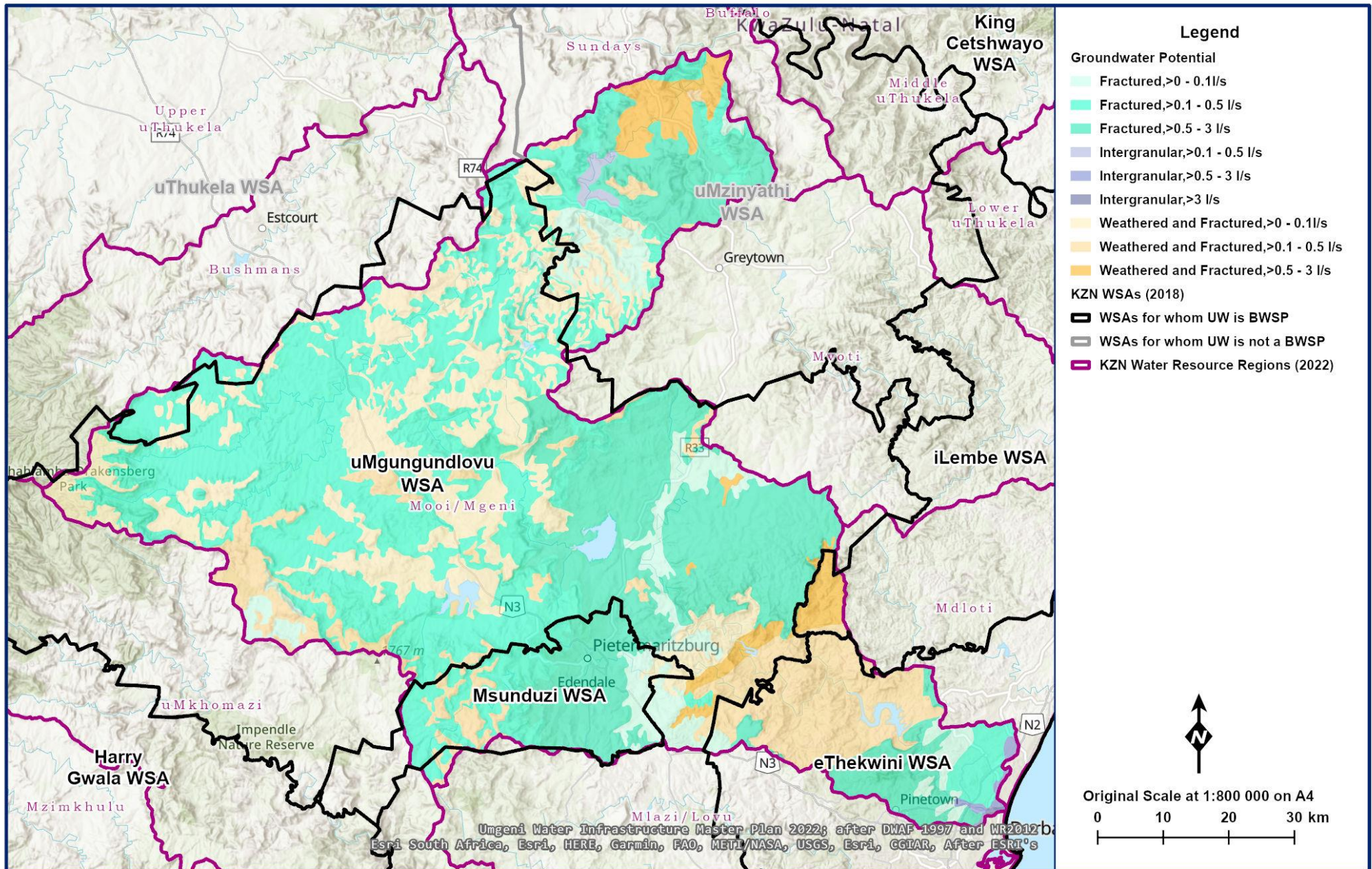
Figure 7.8 Groundwater potential in the Mooi/Mgeni Region (after DWA 1997 and WR2012, MDB 2020, Umgeni Water 2022).
