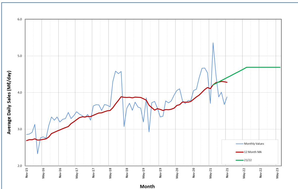
Figure 7.53 Historical demand curve and projections for Maphephethwa WTP.
