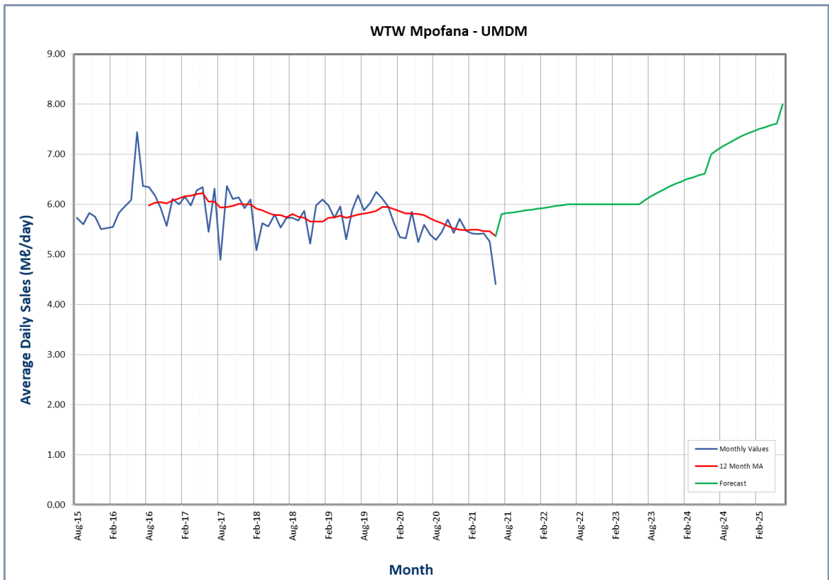
Figure 7.86 Water demand from Mpofana WTP.
