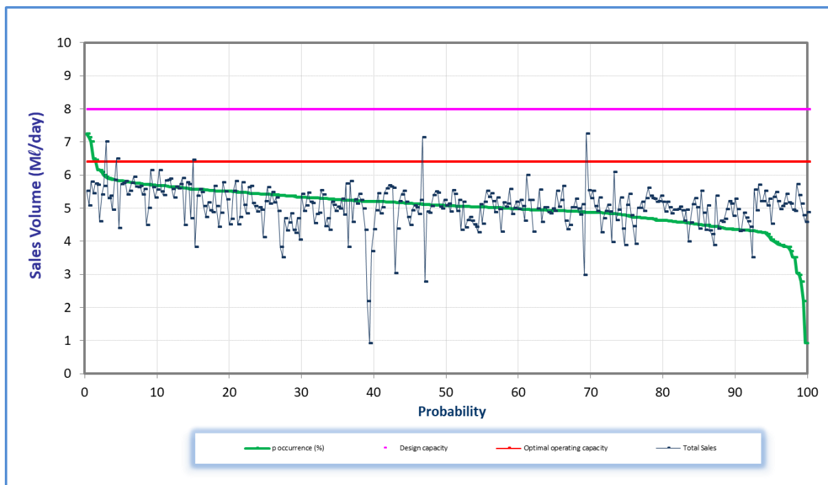
Figure 7.85 Analysis of historical production at Mpofana WTP (November 2019 to October 2020).
