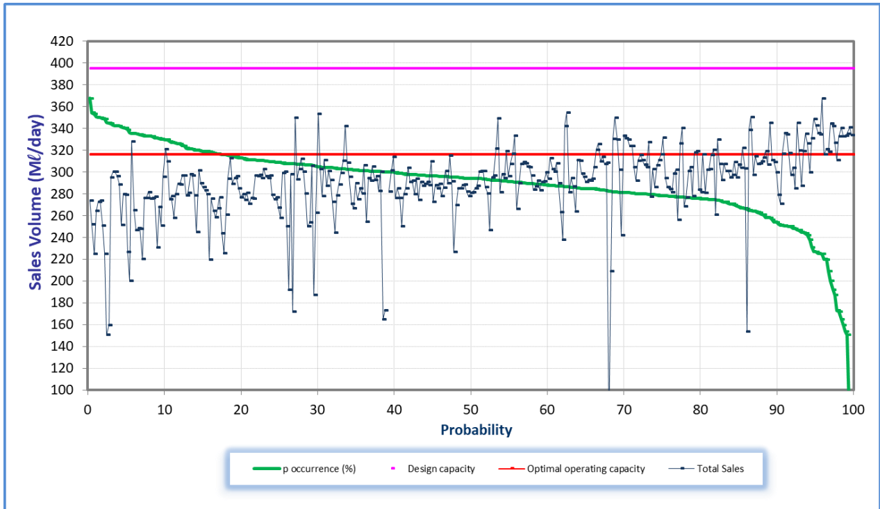
Figure 7.43 Analysis of historical production at Midmar WTP (November 2019 to October 2020).
