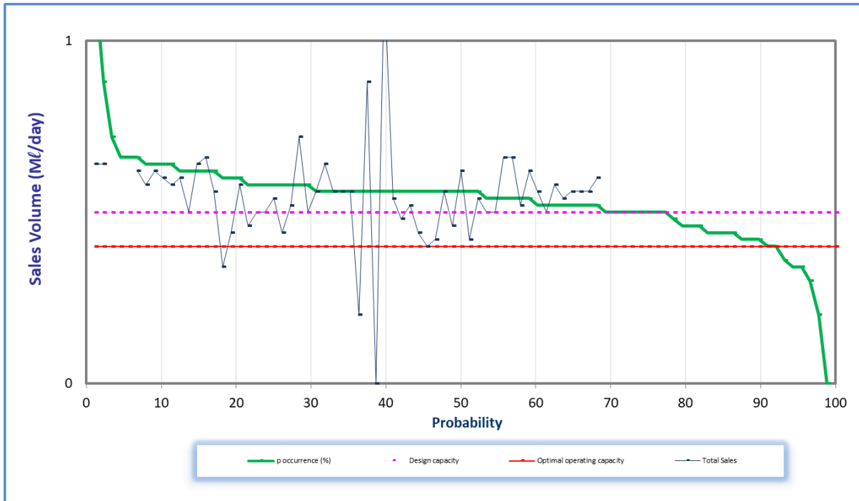
Figure 7.90 Analysis of historical production at Rosetta WTP (November 2019 to October 2020).
