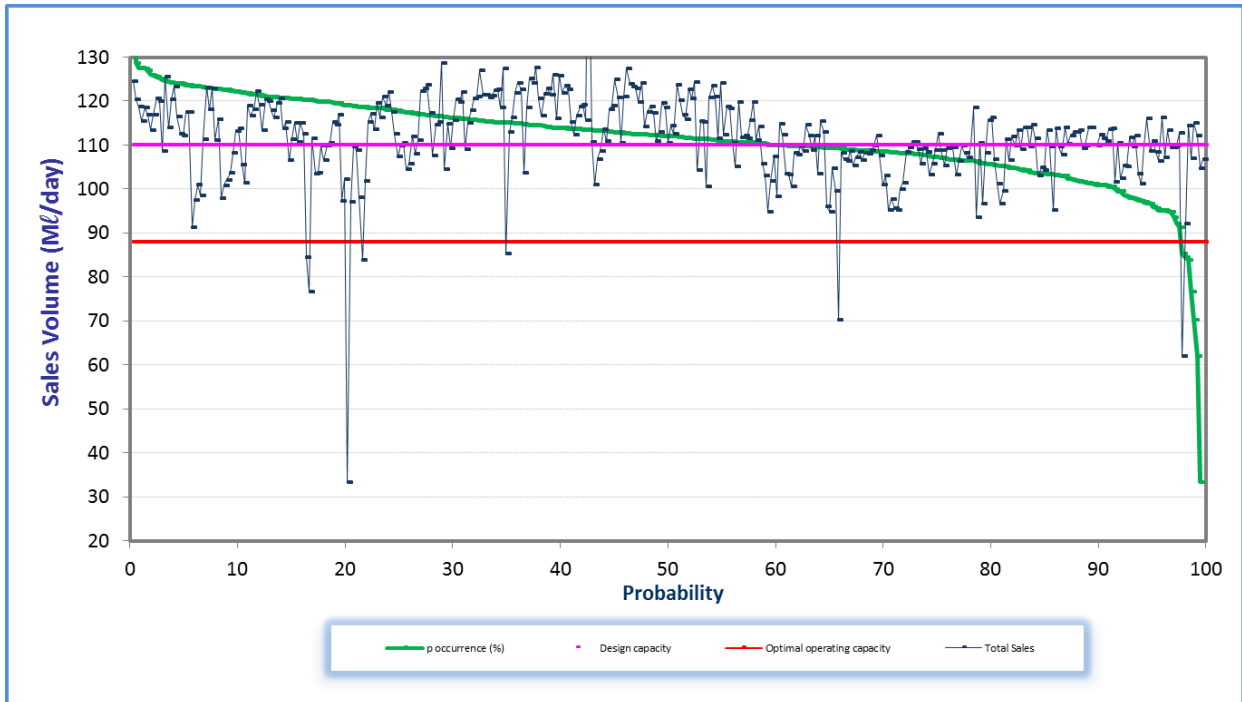
Figure 7.45 Analysis of historical production at D.V. Harris WTP (November 2020 to October 2021).
