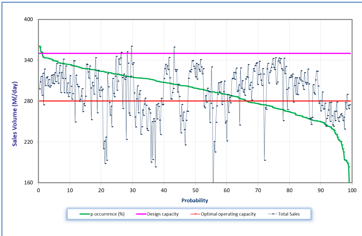
Figure 7.49 Analysis of historical production at Wiggins WTP from November 2020 to October 2021.
