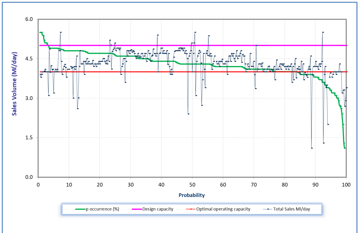
Figure 7.52 Analysis of historical production at Maphephethwa WTP from November 2020 to October 2021.
