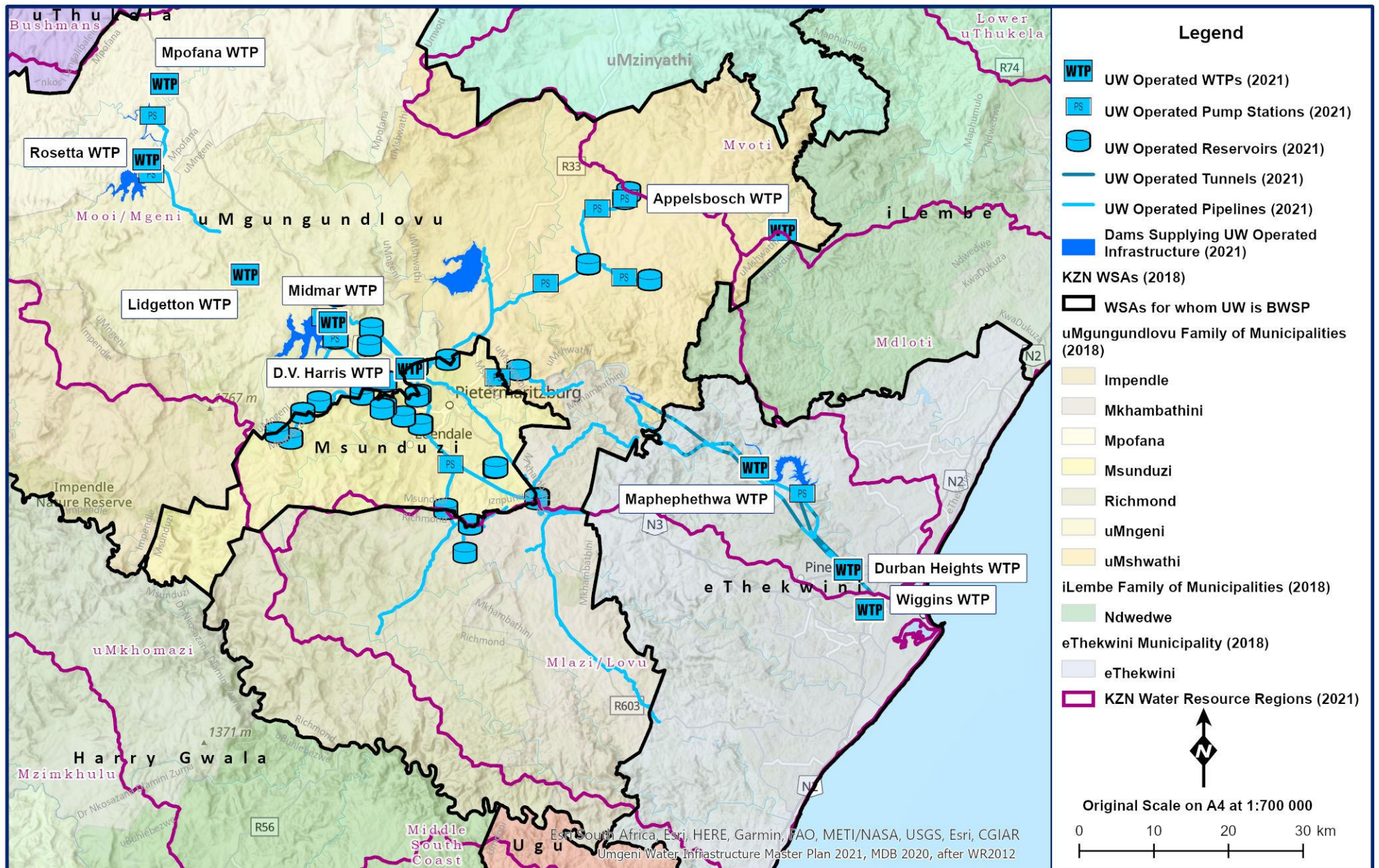
Figure 7.1 General layout of the Mgeni System
