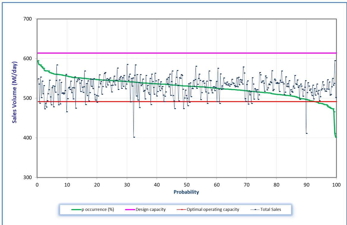
Figure 7.46 Analysis of historical production at Durban Heights WTP from November 2020 to October 2021.
